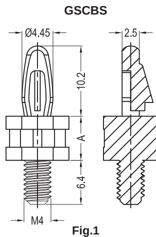
Fig.1 Top Hole: 4.0±0.08mm Panel Thickness: 1.57mm
