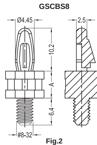
Fig.2 Top Hole: 4.0±0.08mm Panel Thickness: 1.57mm
